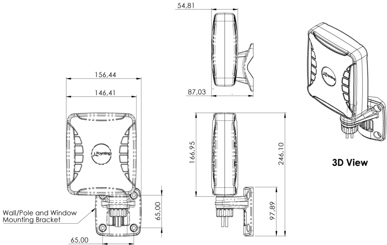
Figure 1; Mechanical drawings
