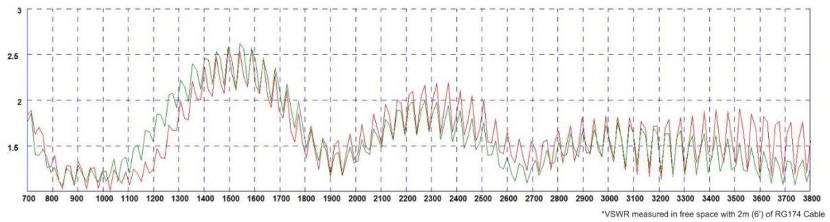
Typical VSWR Elements 1 & 2
