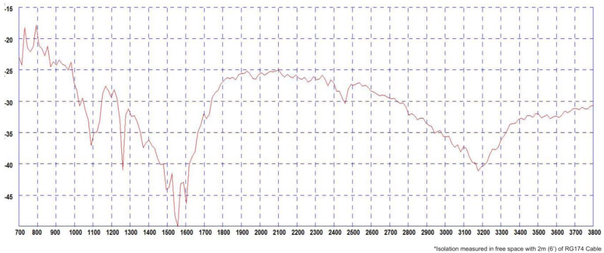
Typical isolation Elements 1 & 2
