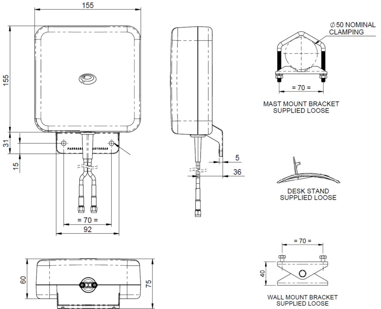
Figure 1; Mechanical drawings
