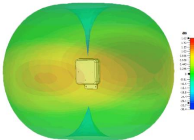
3D Gain Plot (750MHz)
