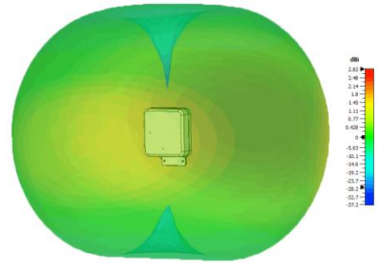
3D Gain Plot (950MHz)
