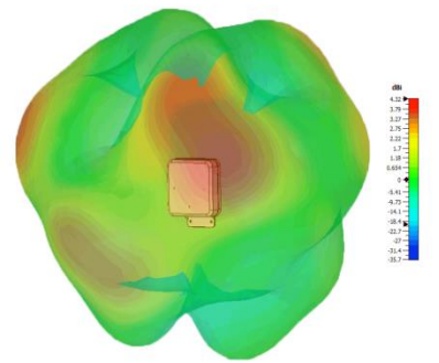
3D Gain Plot (3600MHz)
