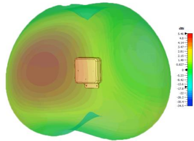
3D Gain Plot (1800MHz)
