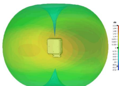
3D Gain Plot (850MHz)
