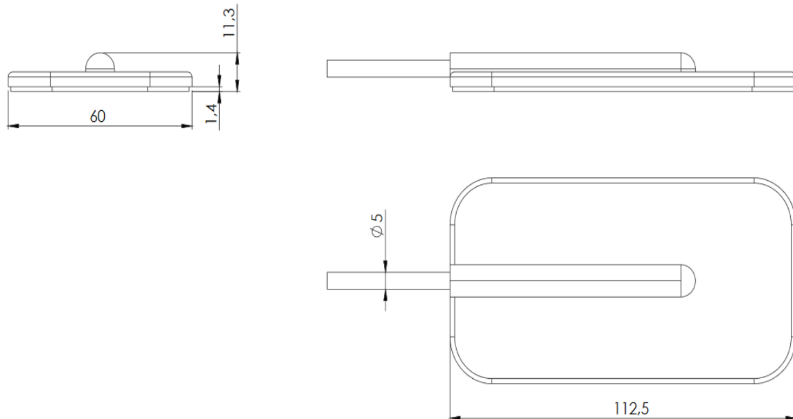
Figure 1; Mechanical drawings
