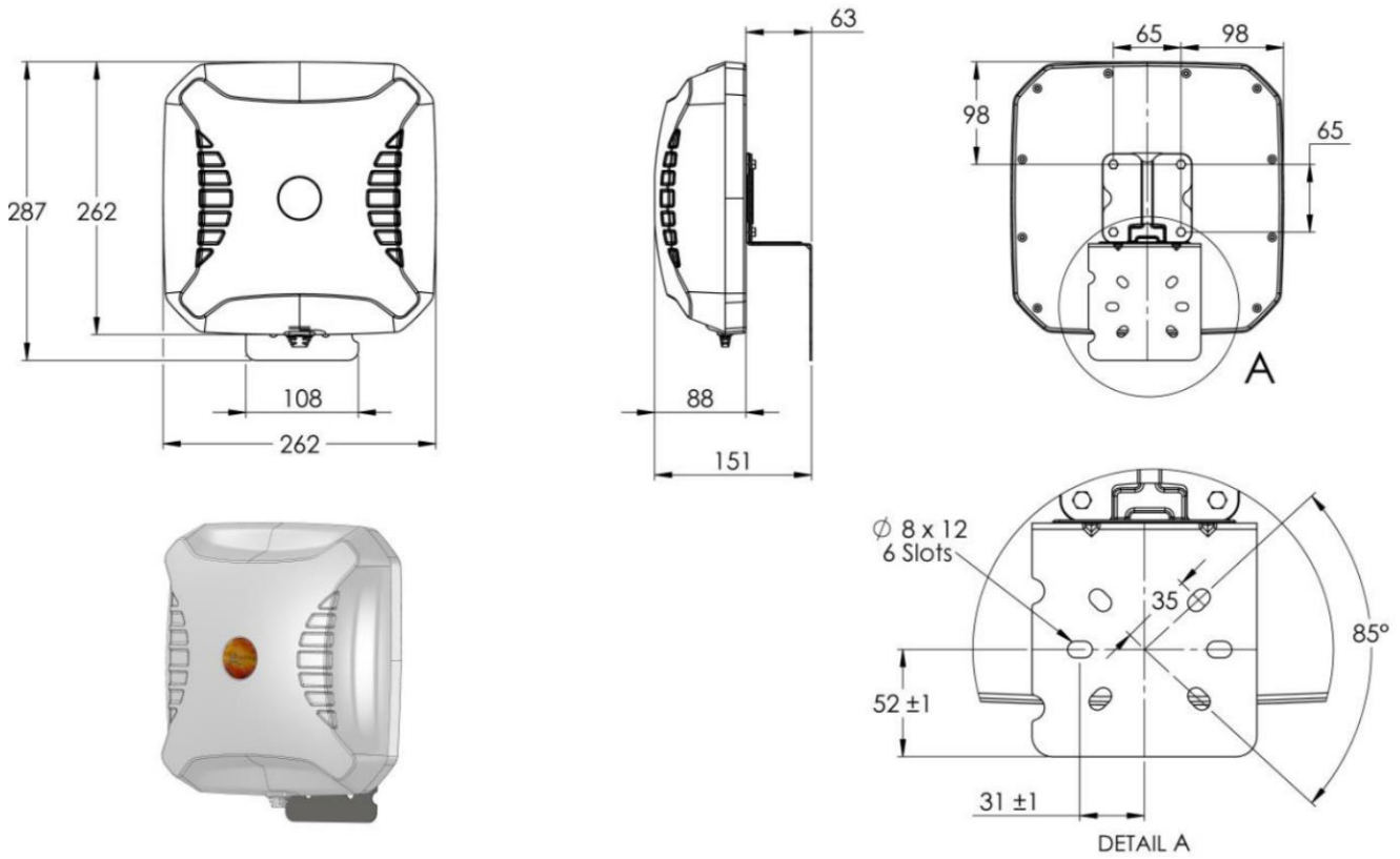
Figure 1; Mechanical drawings
