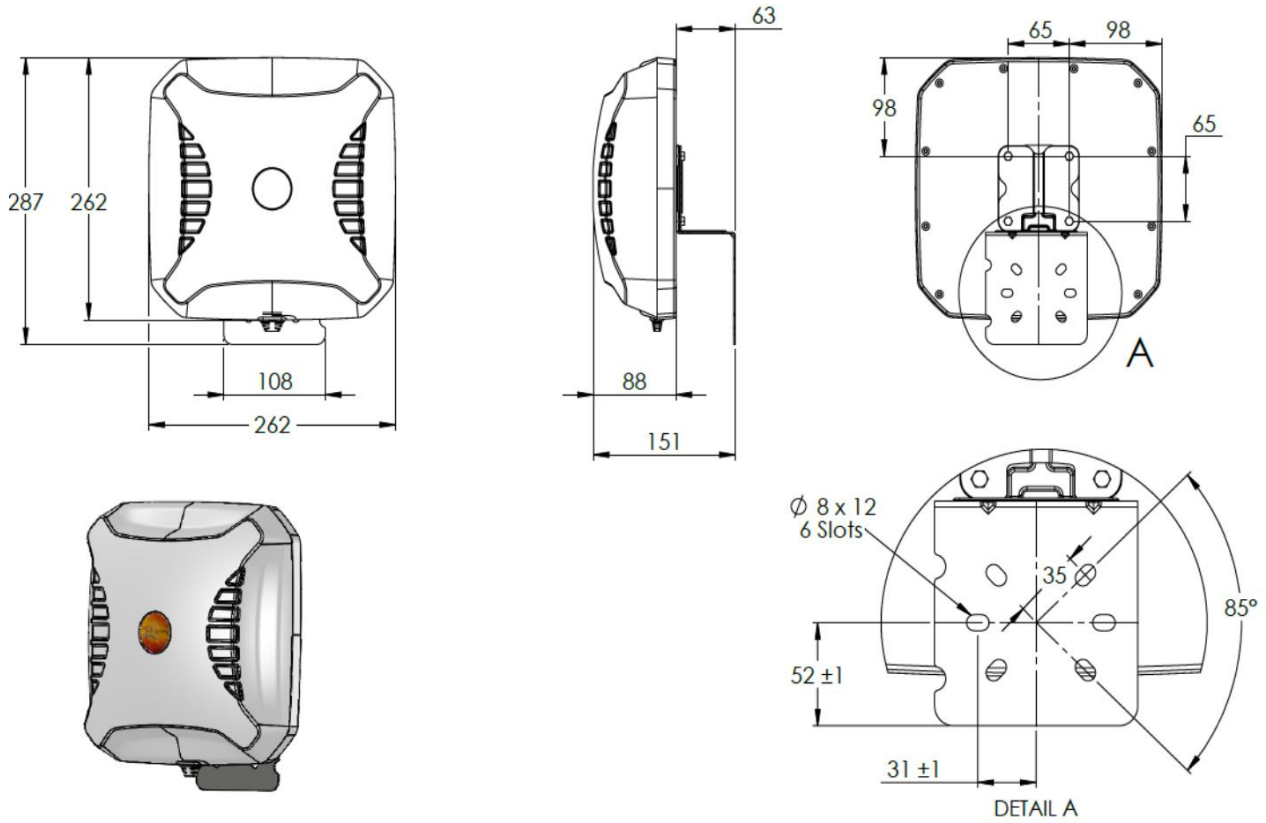
Figure 1; Mechanical drawings
