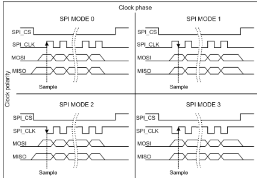
Figure 17.1: SPI modes selectable on SPI
