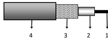
cable detail RG58 (Leoni Dacar 110)
